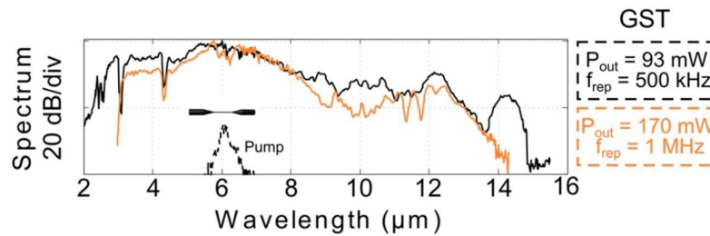
Figure 1: Measured output SC spectra pumped at 6.3 \mu\text{m} for 5-cm-long segment of tapered chalcogenide fiber [Erreur ! Source du renvoi introuvable.].
